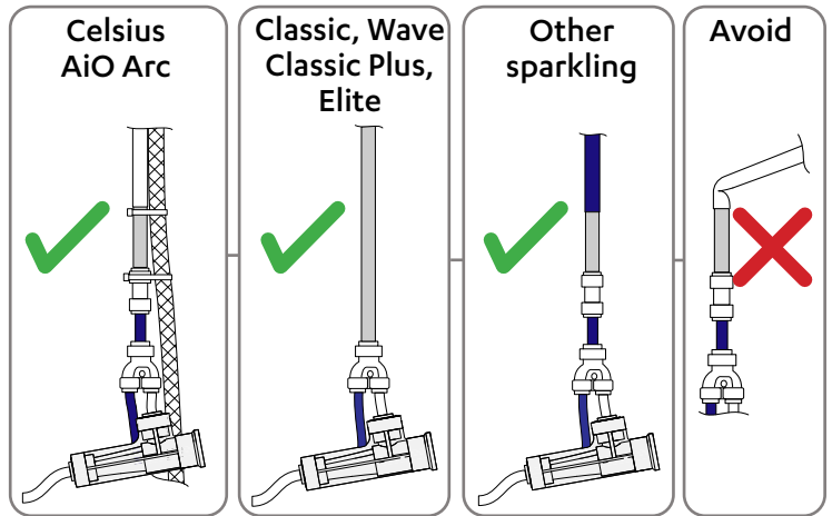
White tube to SPARKLING outlet of Command Centre
